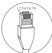
Figure 1-7 Schematic Diagram of Dry Junction Communication Port COM-3
