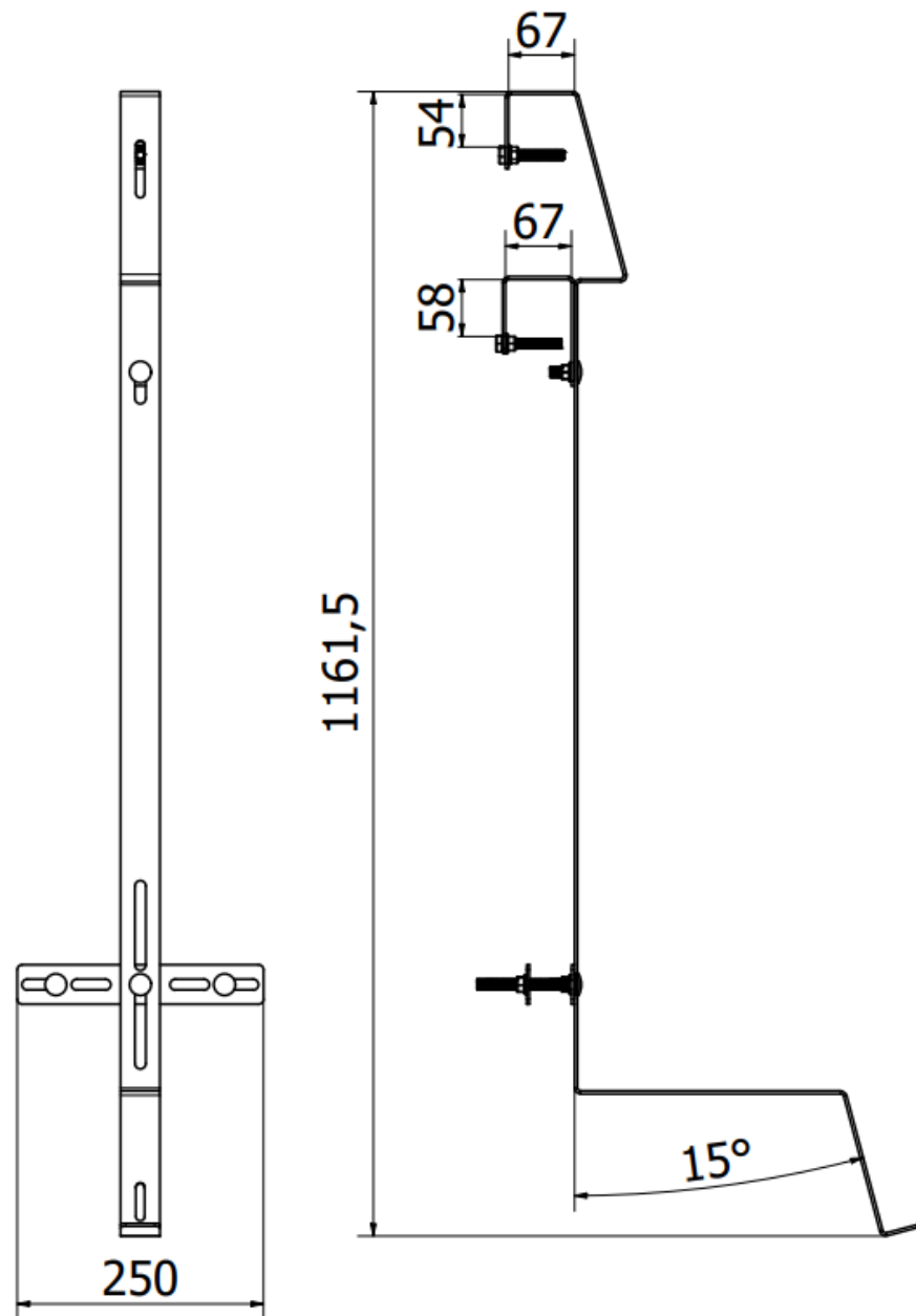
Fig.1 Dimensions of the structure
