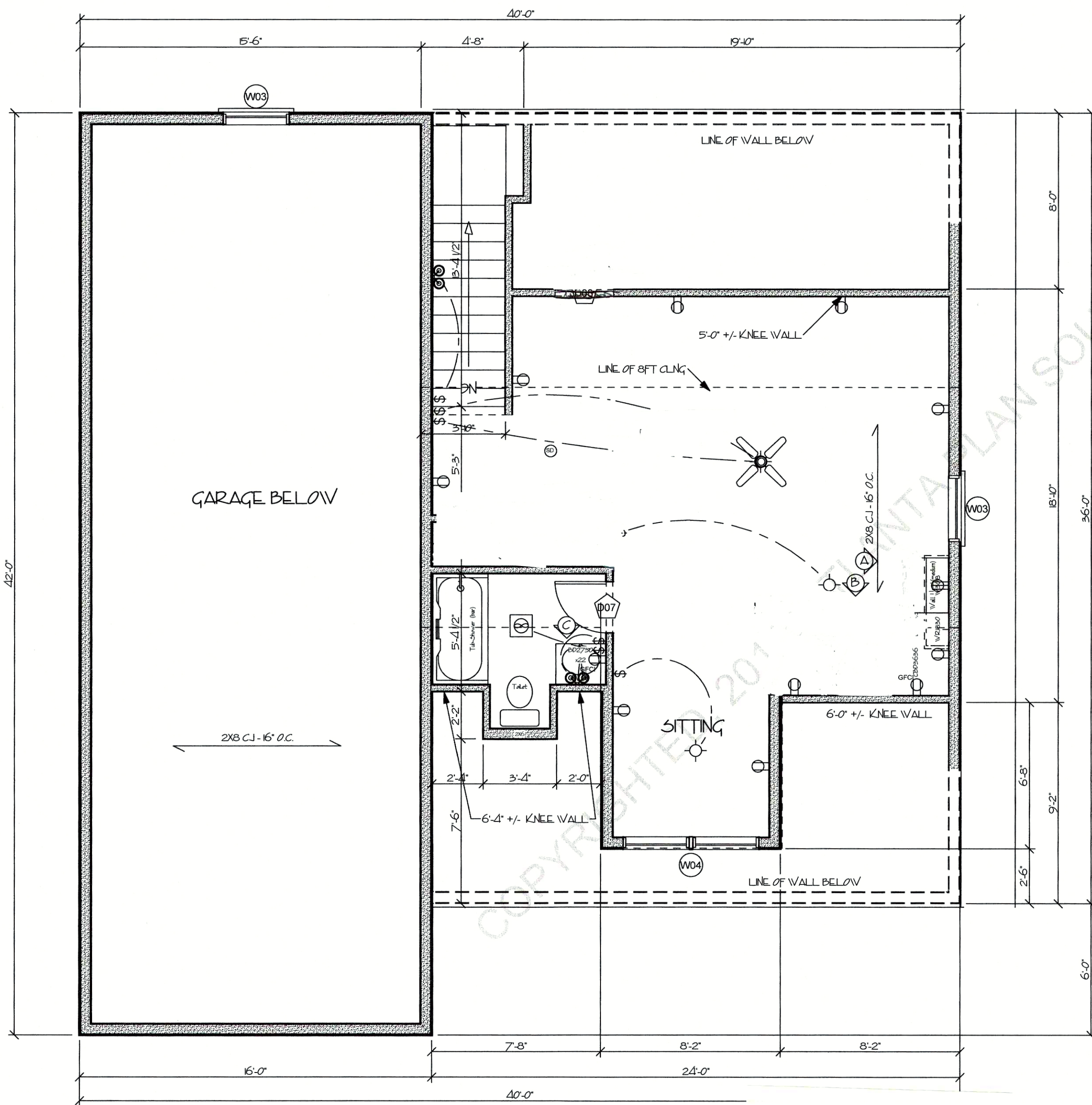
UPPER LEVEL FLOOR PLAN SCALE: 1/4" = 1'-0"
