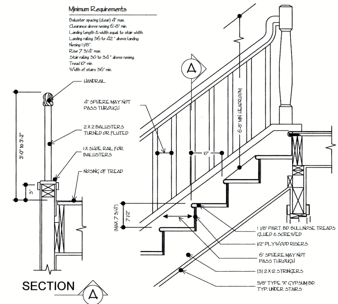
TYPICAL STAIR DETAIL
