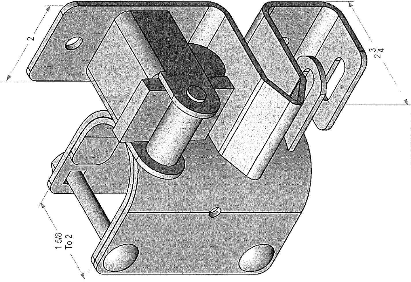
7000-OWR-158-2 2 Round Pin Strap Lockable & One Way Sure Latch Assembly
