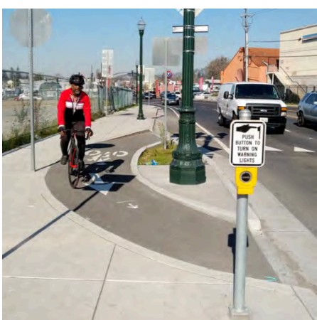
LAMMPS Phase 1
