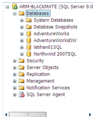
Gambar 12.6. Obyek Databases.
