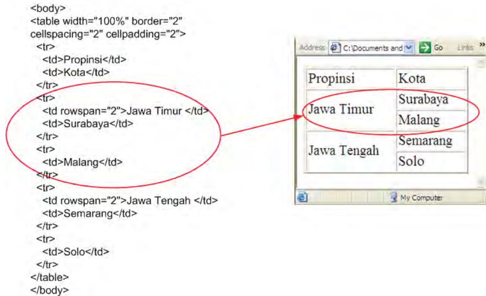
Gambar 13.34. Rowspan.
