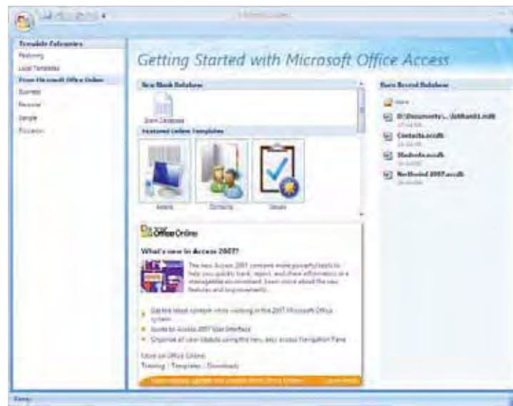
Gambar 11.1. Microsoft Access 2007.
