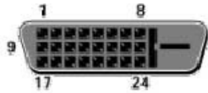
DVI-D Receptacle Connector
