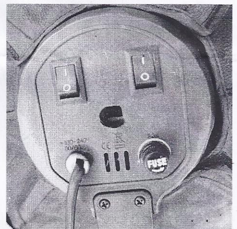
6. Each switch control two lamps, fuse is bundled.
