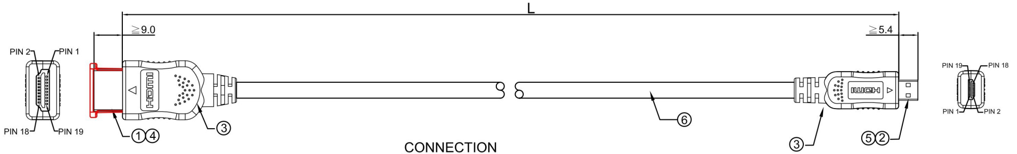
HDMI Type A
