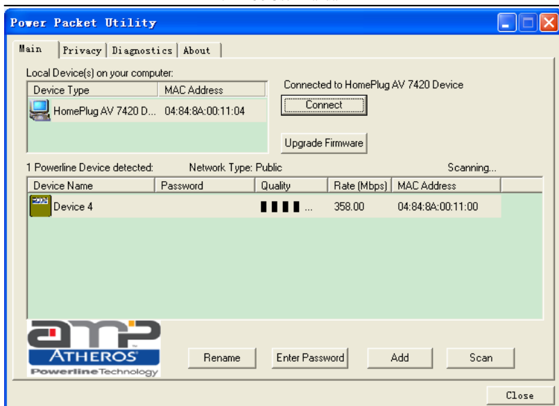
Figure 10 Main Tab
