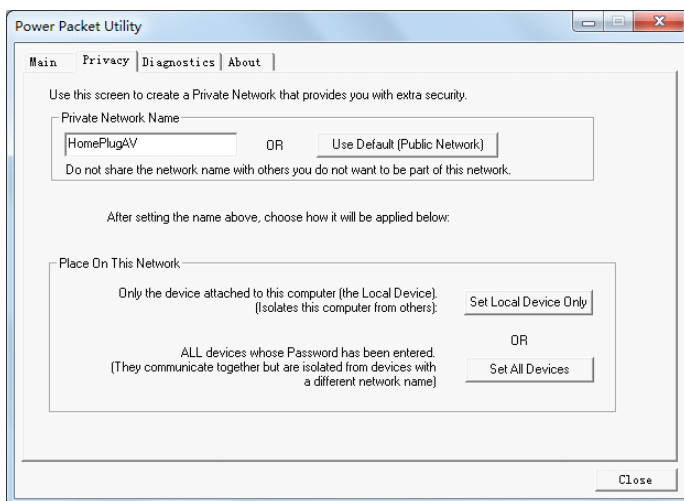
Figure 13 Privacy Tab
