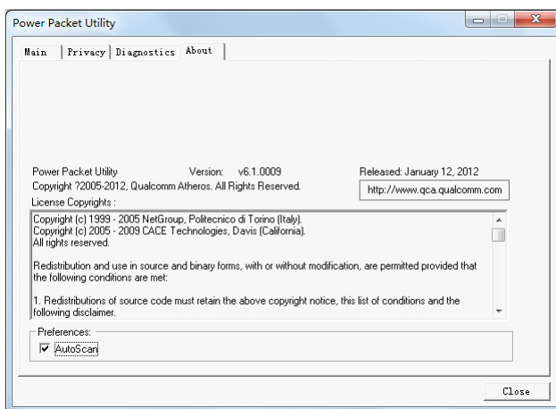
Figure 15 About Tab
