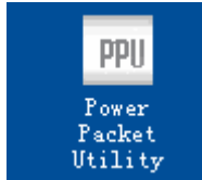
Figure 9 Desktop Icon
