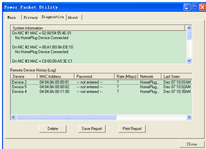
Figure 14 Diagnostics Tab
