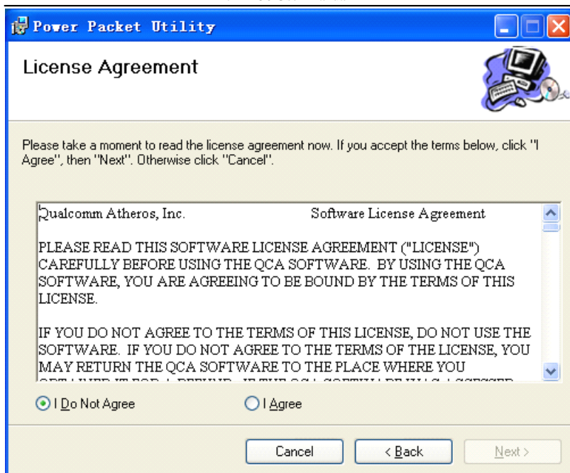
Figure 5 License Agreement
