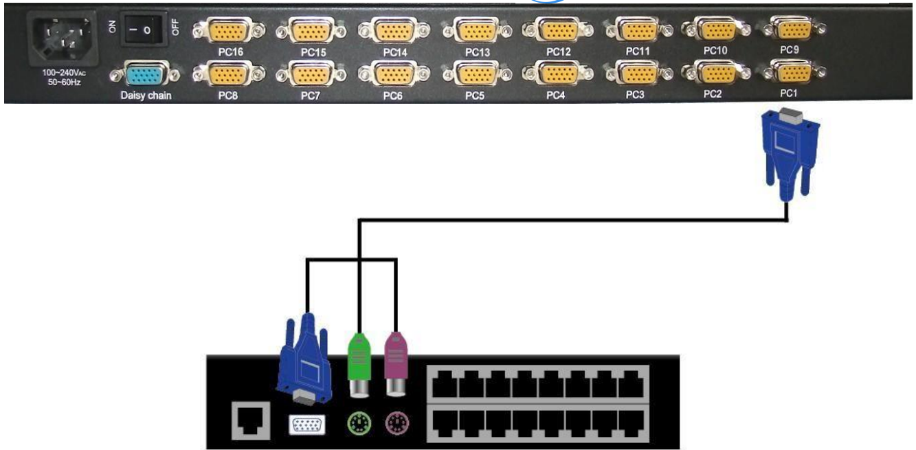
Figure 6. Cascade through Computer Port
