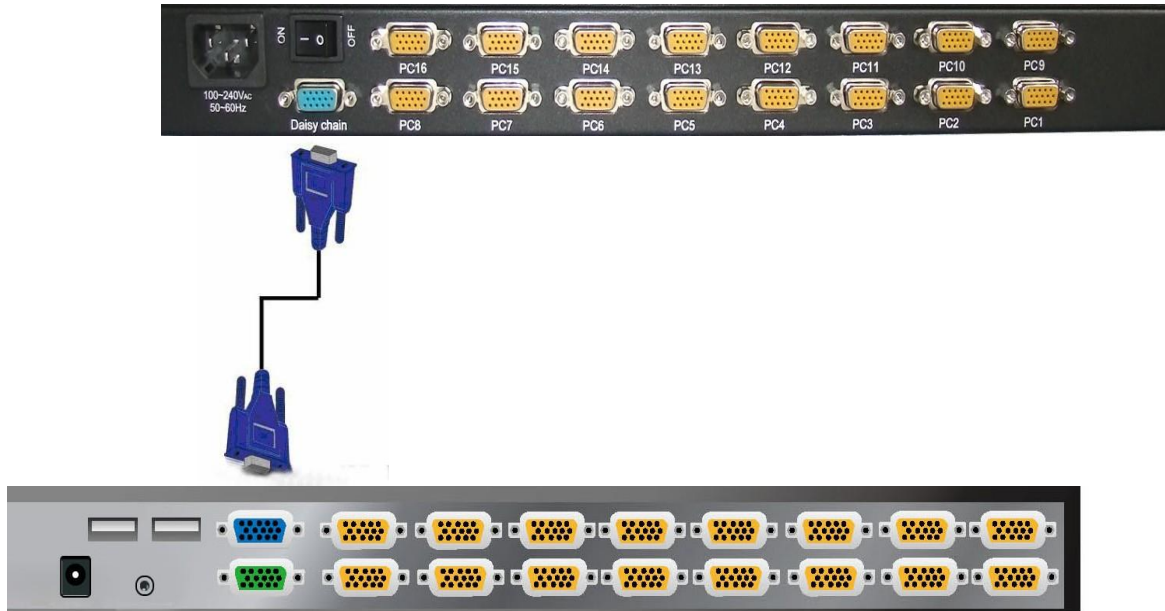
Figure 5. Daisy Chain Connection
