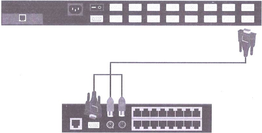
Figure 6. Cascade through Computer Port
