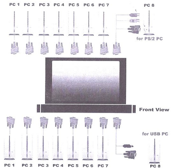
Diagram ( 16 port LCD Drawer )
