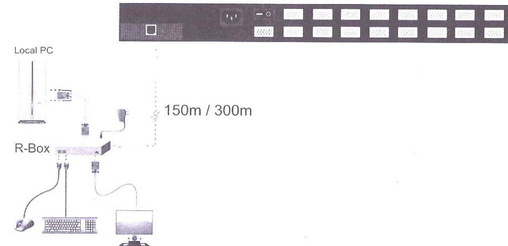
Figure 4. CAT. 5 Module Diagram
