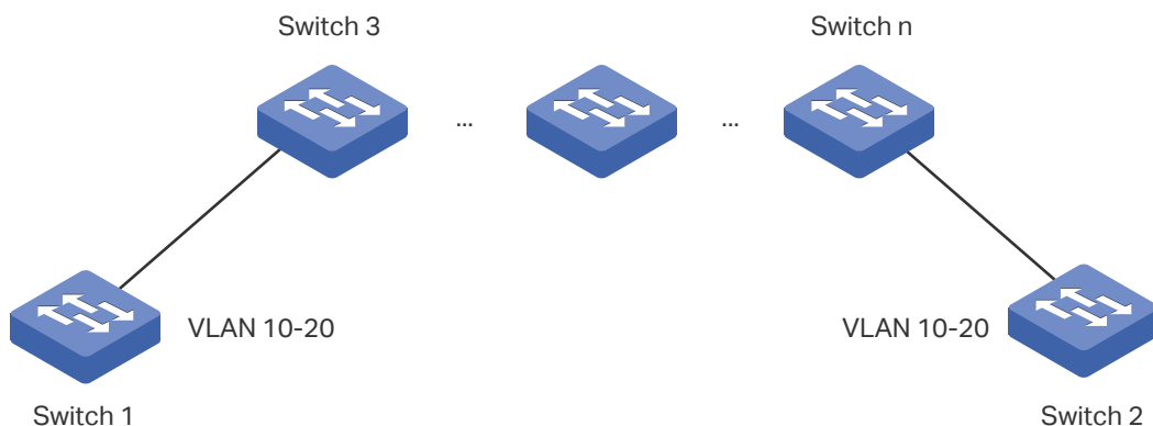
Figure 1-2 GVRP Topology
