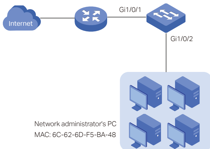
Figure 3-23 Network Topology
