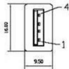
USB A MALE
