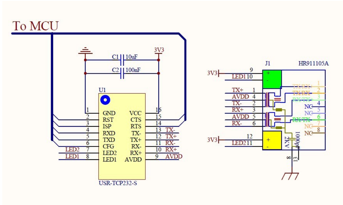
USR-TCP232-S+RJ45 of built-in network transformer:
