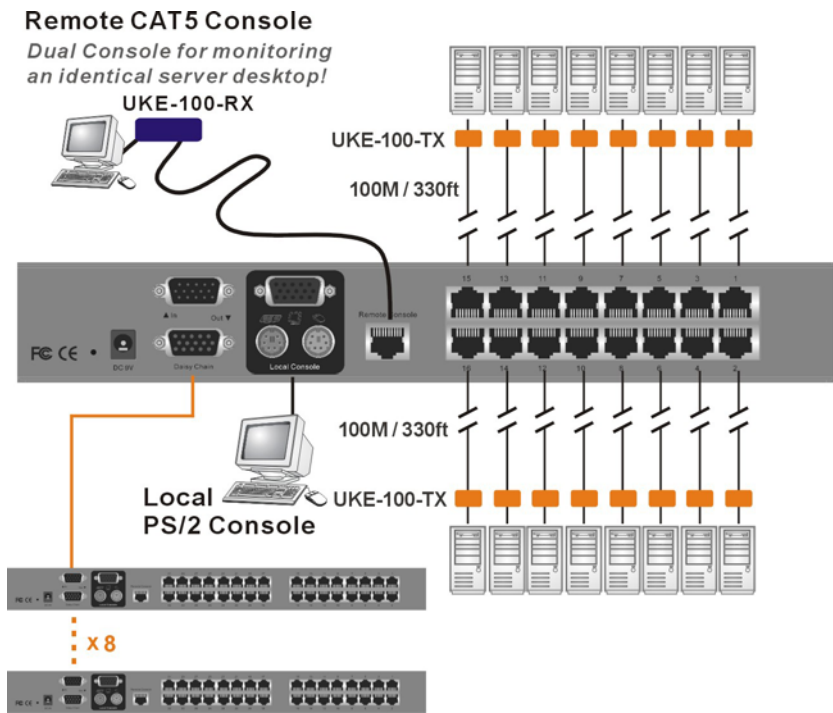
Configuration Diagram (showing UKS-0116OSD and UKS-0132OSD)
