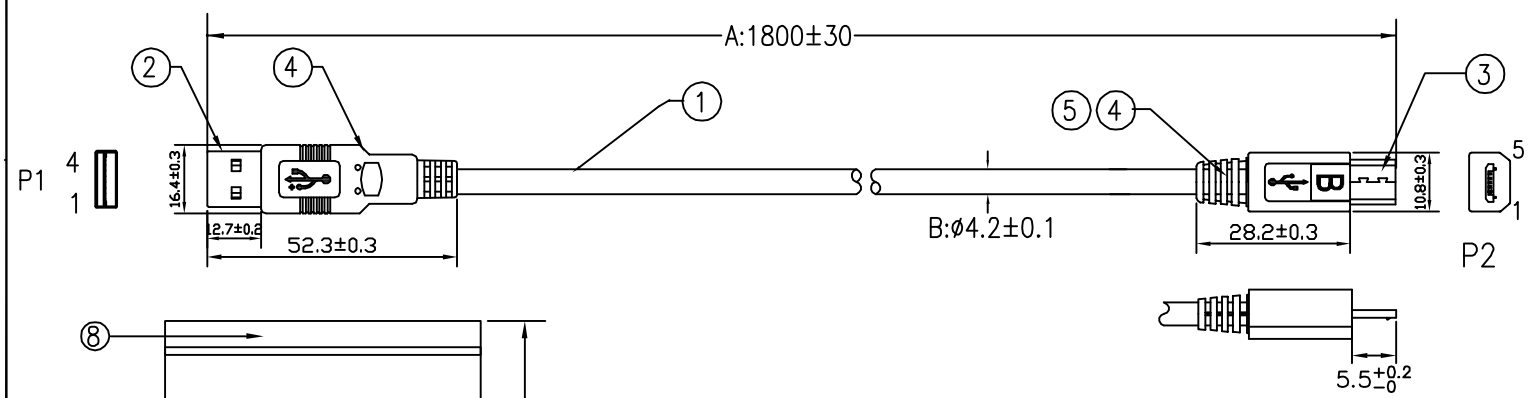
MICRO USB B PLUG
