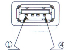
USB-A FEMALE
