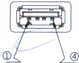
USB-A FEMALE
