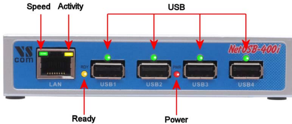
Figure 45: USBIP LED
