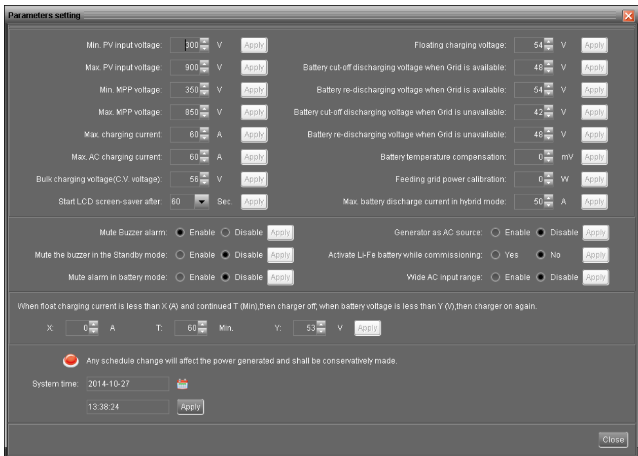
Diagram 4-11C (Off-Grid mode)
