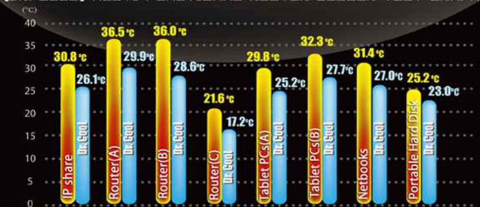
[DR. COOL] MULTI FUNCTIONAL ROUTER COOLER TEST GRAPH
