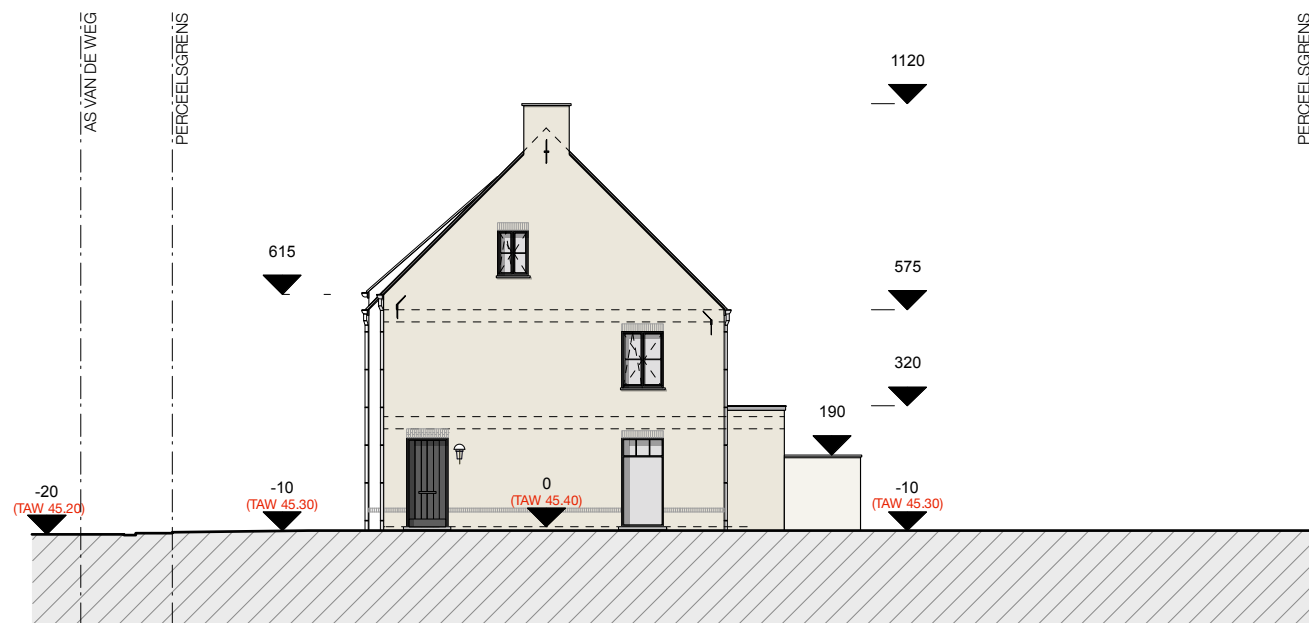
WONING LOT 6
