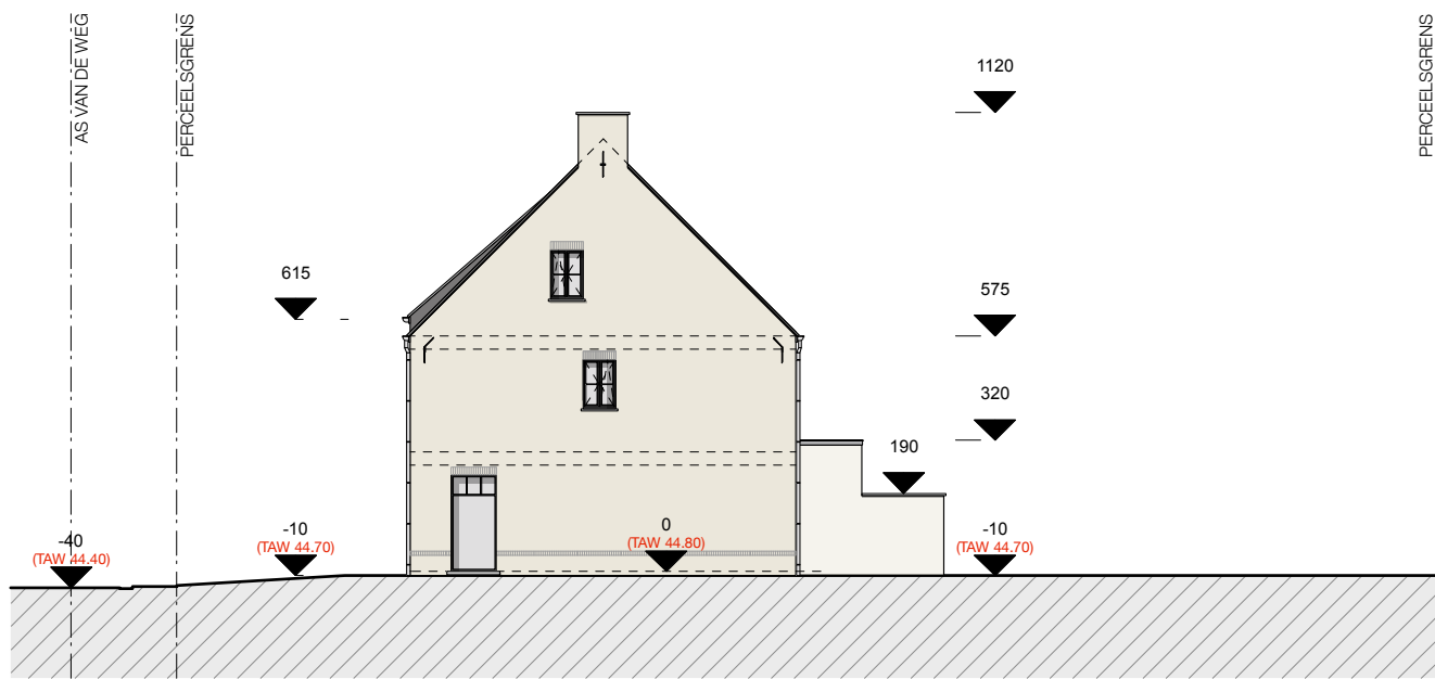
WONING LOT 2
