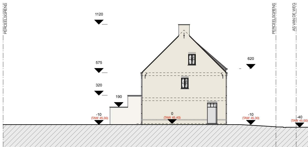
WONING LOT 5
