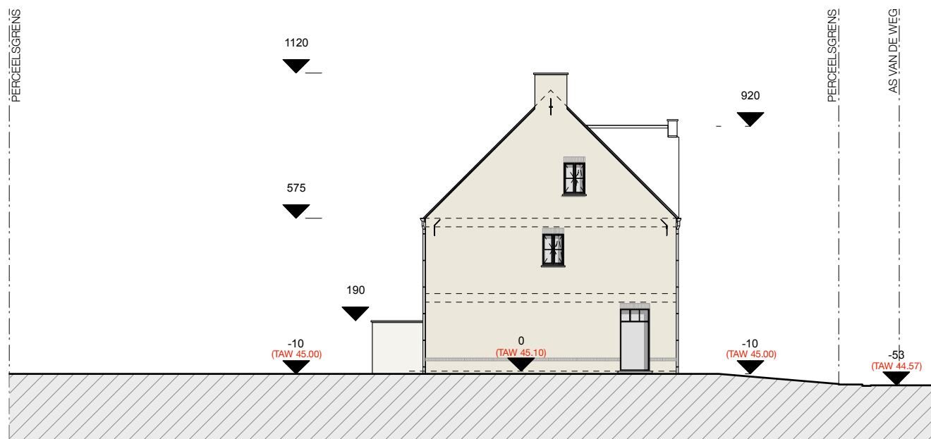
WONING LOT 3
