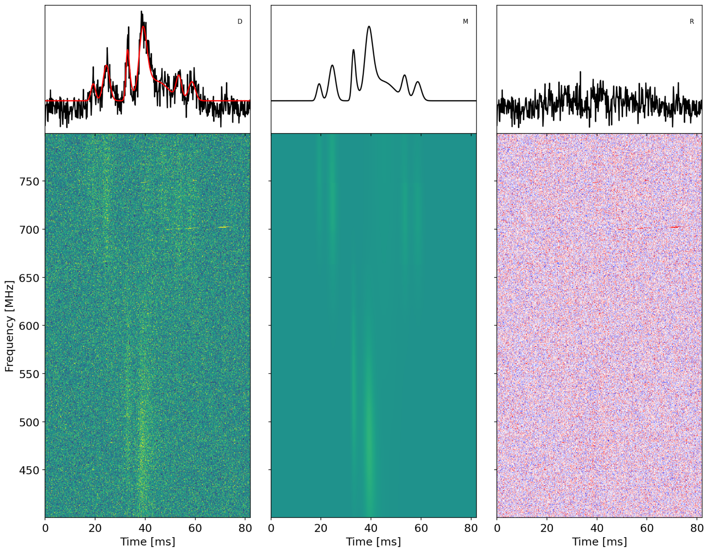
Waterfall plot showing the brightest burst at the reported DM (left), a multicomponent model fitted to extract the burst parameters (CHIME/FRB Collaboration 2021, ApJs, 257, 59; middle), and the residual plot (right). The burst was coherently dedispersed using voltage data recorded at a time resolution of 160 microseconds.
