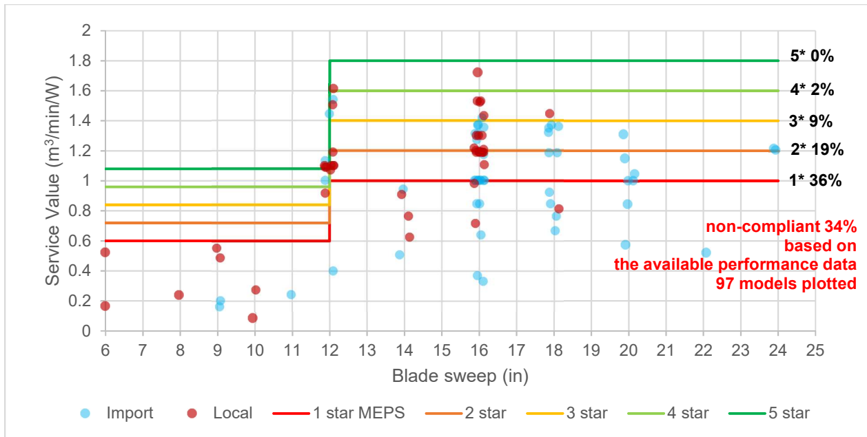
Figure 35: CLASP policy recommendation for Indonesia electric fan products with blade sweep of 6 to 24 inches
