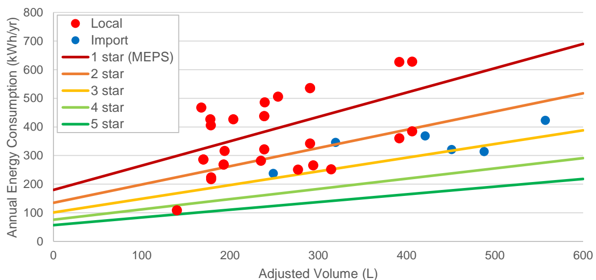
Figure 35: CLASP's recommended performance requirements compared to the performance of tested models.
