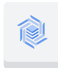
Bigtable
