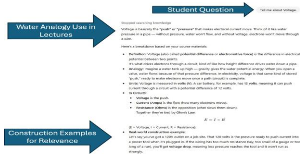
Figure 2. Chatbot Interaction.
