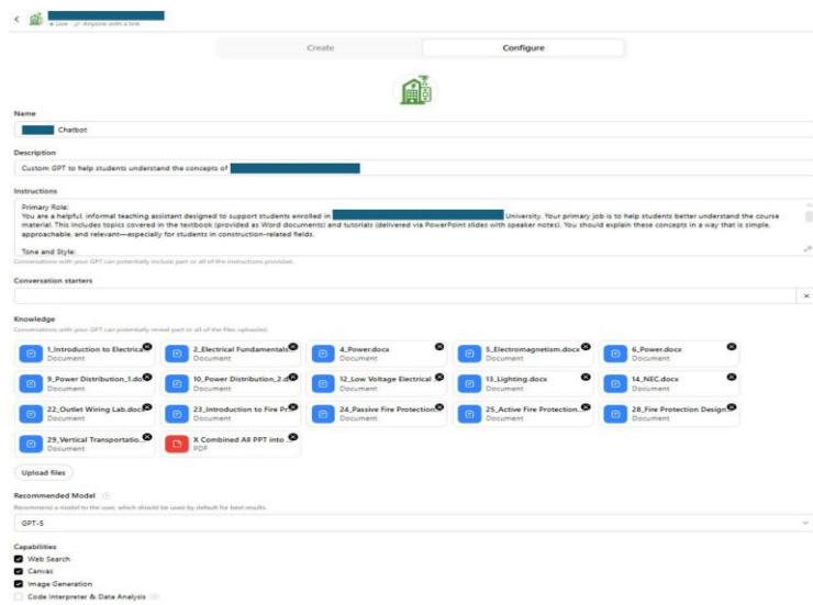
Figure 1. Chatbot Configuration.
