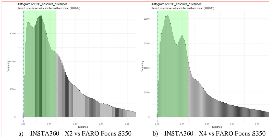
Figure 5. Cloud-to-cloud (C2C) distance visualizations and histograms
