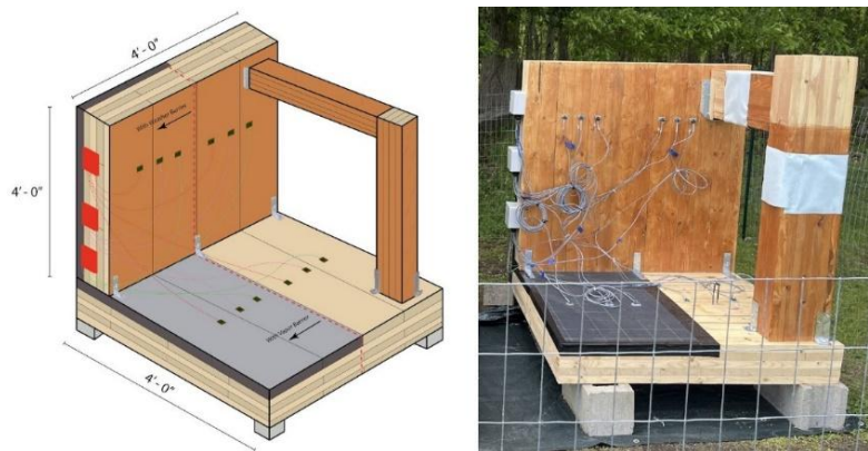
Figure 1. The CLT Mock-up and Sensors Attachment Details
