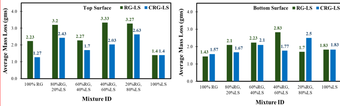
Figure 2. Average mass loss comparison between different mixtures for a) top surface and b) bottom surface of concrete specimens.
