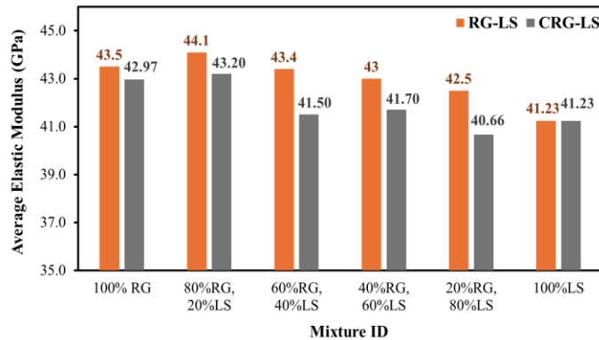
Figure 5. Average values of dynamic elastic modulus per mixture for different mixture composition
