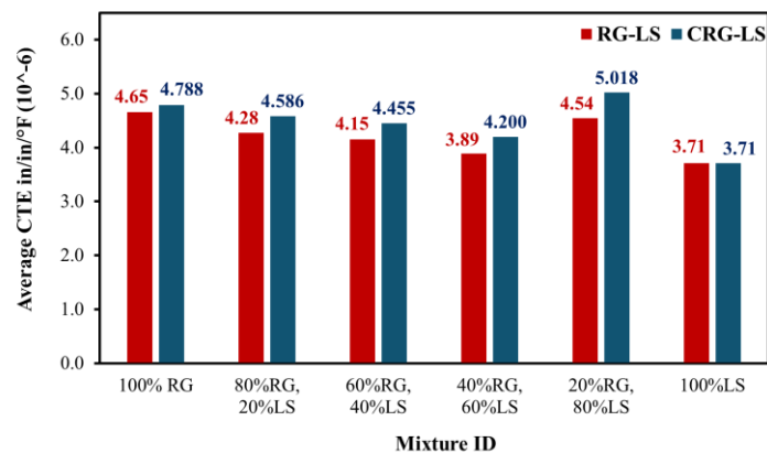
Figure 4. Average value of Coefficient of Thermal Expansion per mixture for different mixture composition
