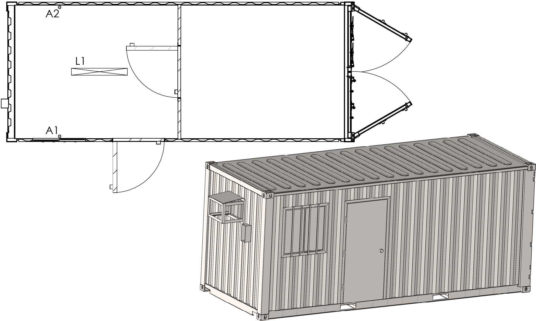
ELECTRIC PLAN
