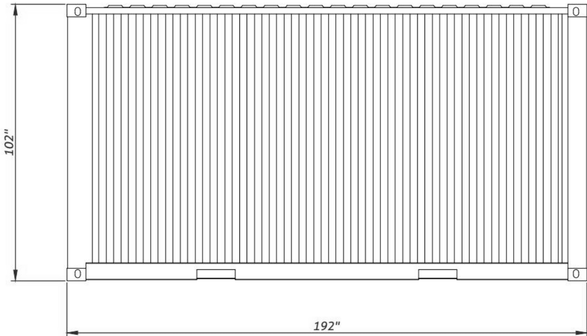
● Right view
