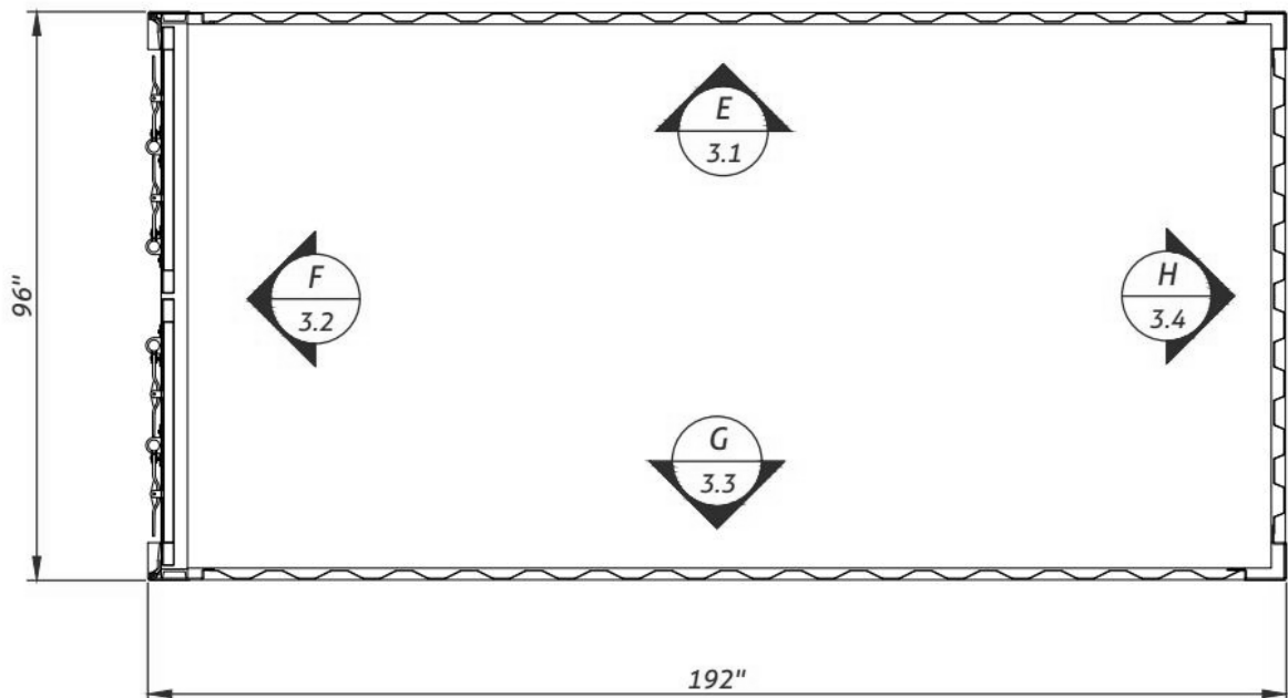
● Floor view
