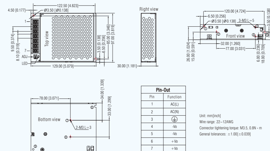
LM100-20/22Bxx Series: LxWxH:129×97×30(mm)
