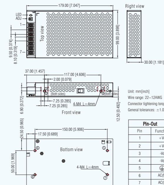
1 LM200-10Bxx Series: LxWxH:179x99x30(mm)
