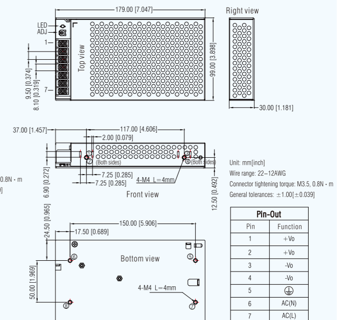
2 LM200-12Bxx Series: LxWxH:179x99x30(mm)
