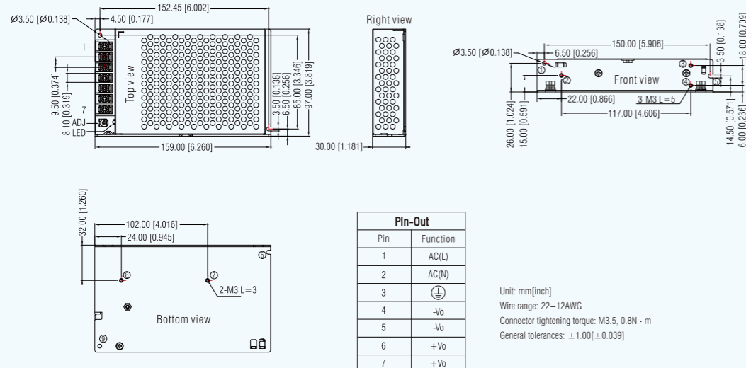
LM150-20/22Bxx Series: LxWxH:159x97x30(mm)
