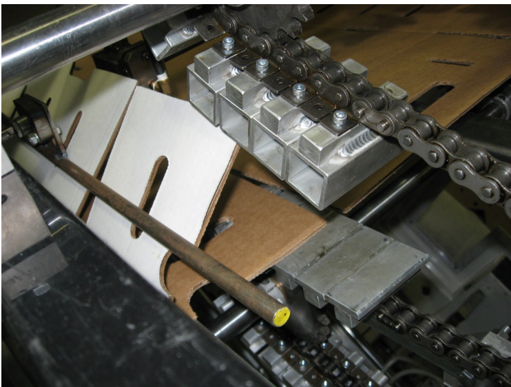
LAMINATING MODULE
