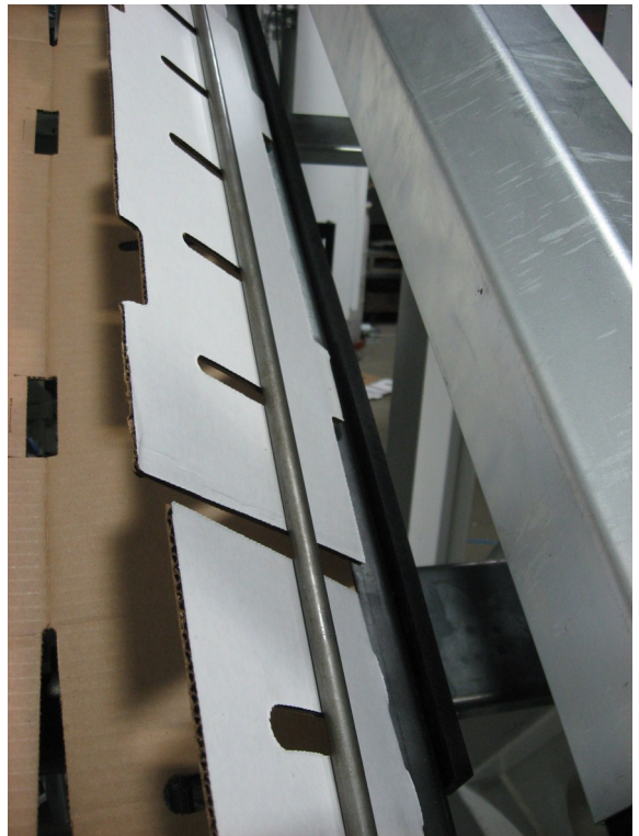
SECONDARY PLOW
