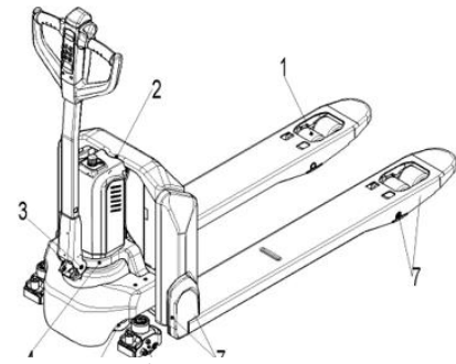
Figure 13: Lubrication points
