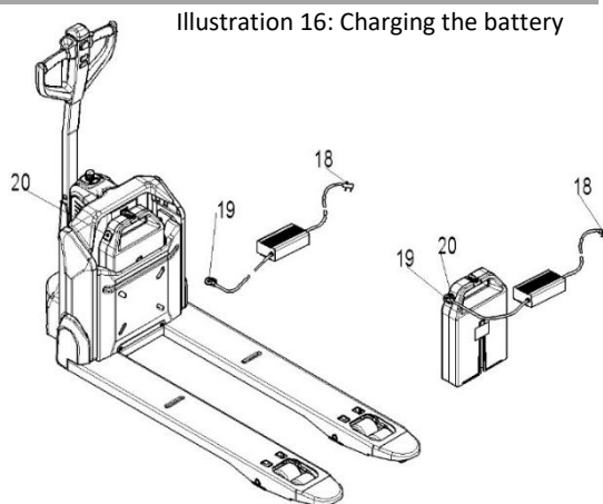
Illustration 16: Charging the battery
