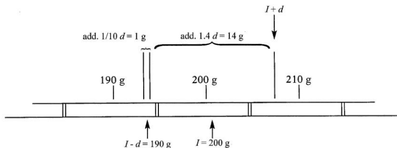
Figure 10 – Instrument with d = 10 g
