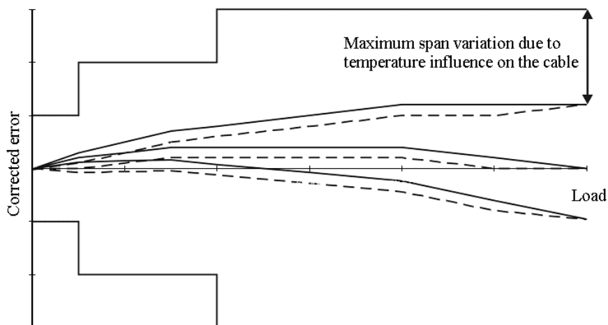
Figure 12 – Span variation
