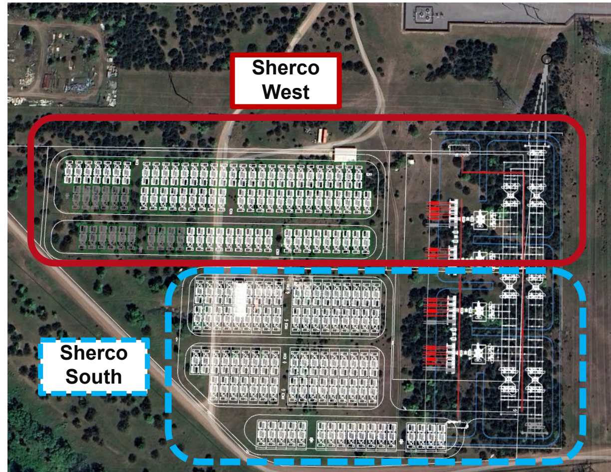
Figure 1 – Image Represents Preliminary Site Layout
