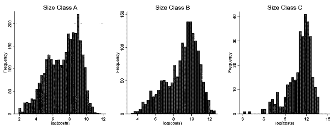
Fig 6. The distribution of \log(\text{costs}) , by size class.
