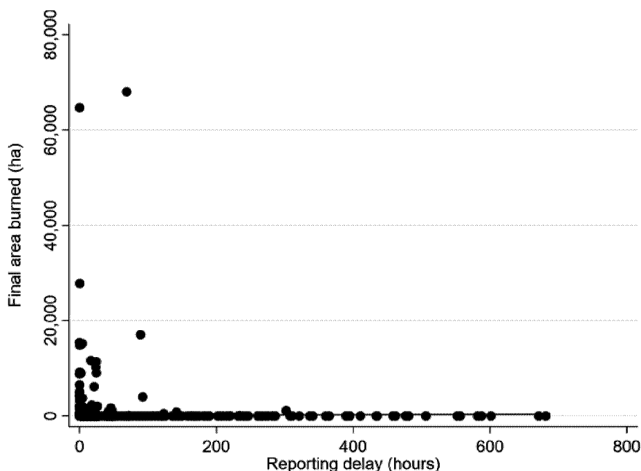
Fig 5. Scatter plot of final area burned and reporting delay.
