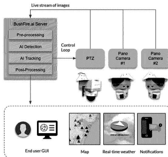
Figure 3 System architecture
