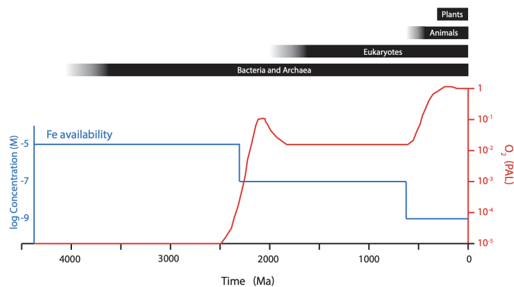
Figure 1: Great Oxidation Event. See [Knoll and Nowak, 2017].
