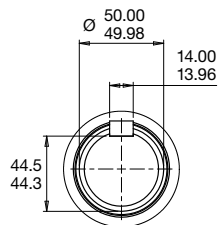
SHAFT END DETAIL
