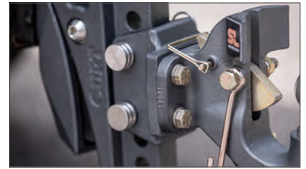
Pintle mount accepts any CURT mount-style pintle hook or combination hitch
