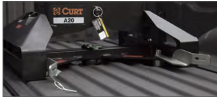
Step 1 - Drop OEM product into the truck bed puck system
