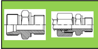
UNION MACHO BSPP
