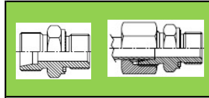
UNION MACHO BSPP C/JUNTA
