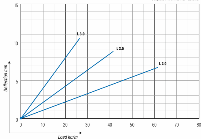
KRA/KRB 40 | WIDTHS 100, 200
