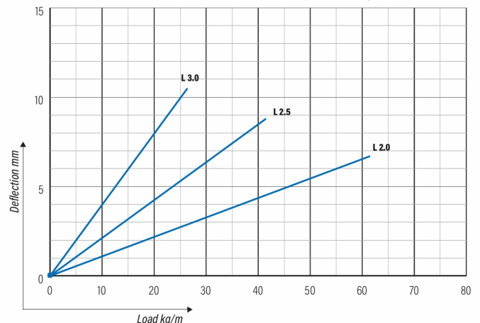
KRA/KRB 40 | WIDTHS 100, 200
