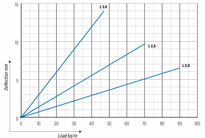
KRA/KRB 40 | WIDTHS 400, 500, 600
