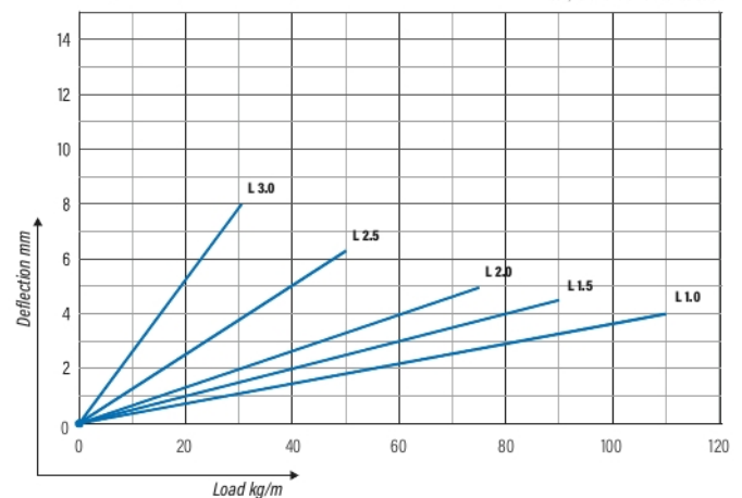
KRA/KRB 60 | WIDTHS 100, 200
