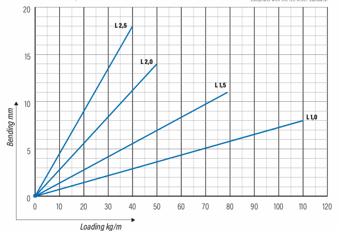
WMT 100 | WIDTHS 300, 400, 500, 600
