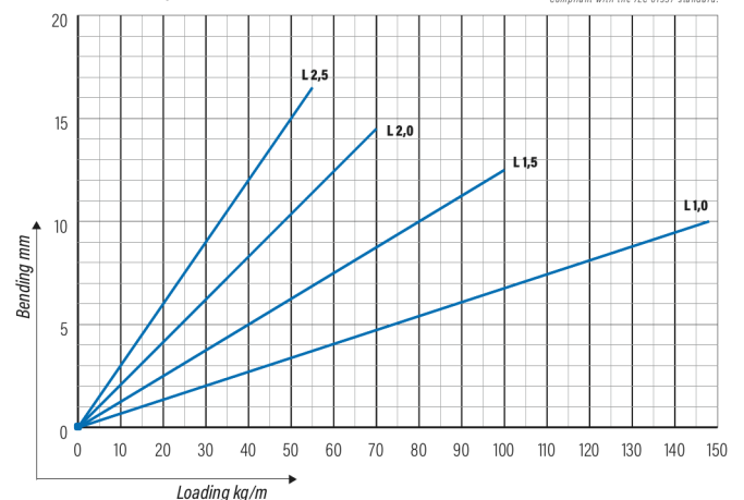
WMT 150 | WIDTHS 300, 400, 500, 600
