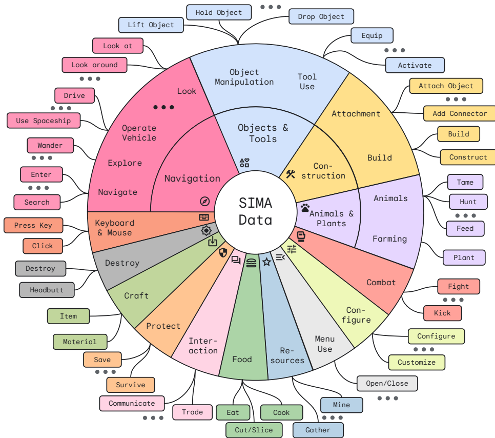
Figure 3 | Instructions Across SIMA Data. The SIMA dataset includes a broad range of text instructions that can be roughly clustered into a hierarchy. Due to the common 3D embodied nature of the environments that we consider, many generic tasks, such as navigation and object manipulation, are present in multiple environments. Categories were derived from a data-driven hierarchical clustering analysis of the human-generated text instructions within a fixed, pretrained word embedding space. Note that the area of each cluster in the wheel in Figure 3 does not correspond to the exact number of instructions from that cluster in the dataset.
