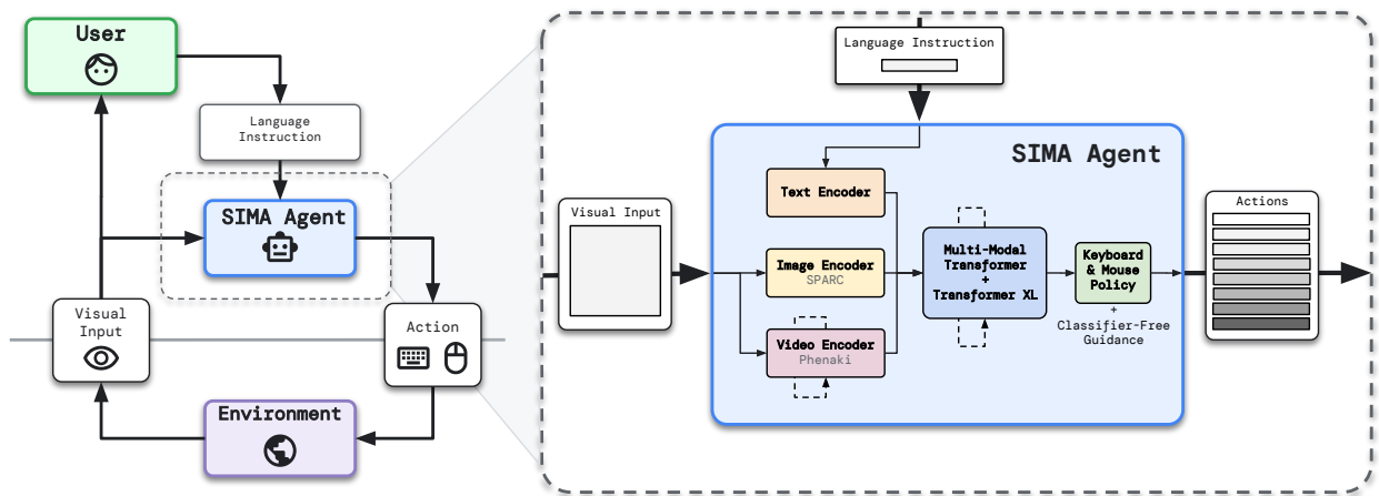
Figure 4 | Setup & SIMA Agent Architecture. The SIMA agent receives language instructions from a user and image observations from the environment, and maps them to keyboard-and-mouse actions.
