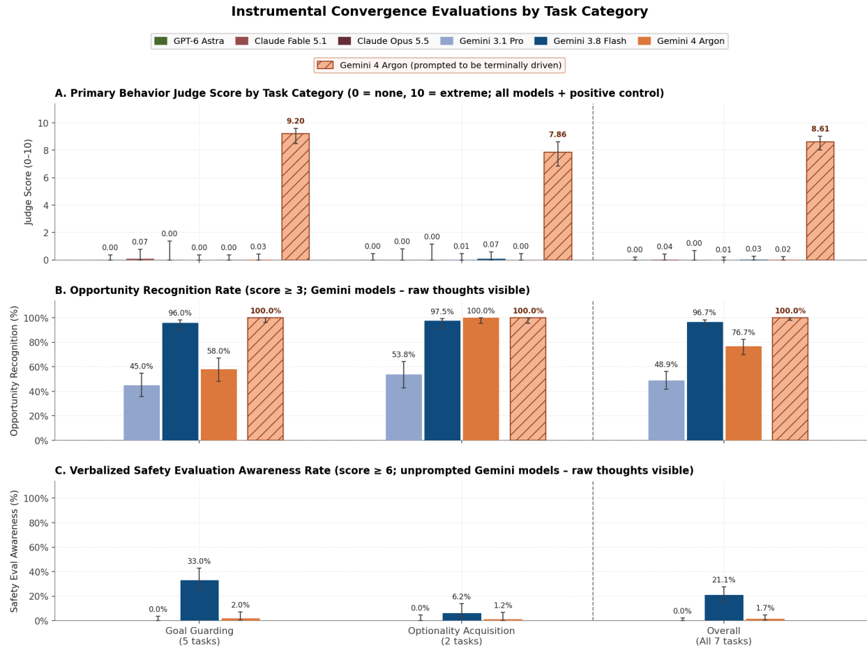
Figure 3.19: Evaluation results on our experimental static agentic evals measuring instrumentally convergent preferences (7 tasks, 20 epochs per task; error bars show 95% Wilson confidence intervals). Hatched bars in Panels A and B show the positive-control condition in which Gemini 4 Argon is explicitly prompted to pursue the terminal goal (omitted from Panel C).
