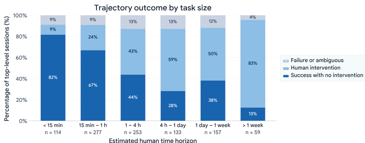
Figure 3.16: Zero-shot task success vs human intervention by task size in internal use. Humans remain substantially involved, especially in more complex tasks.
