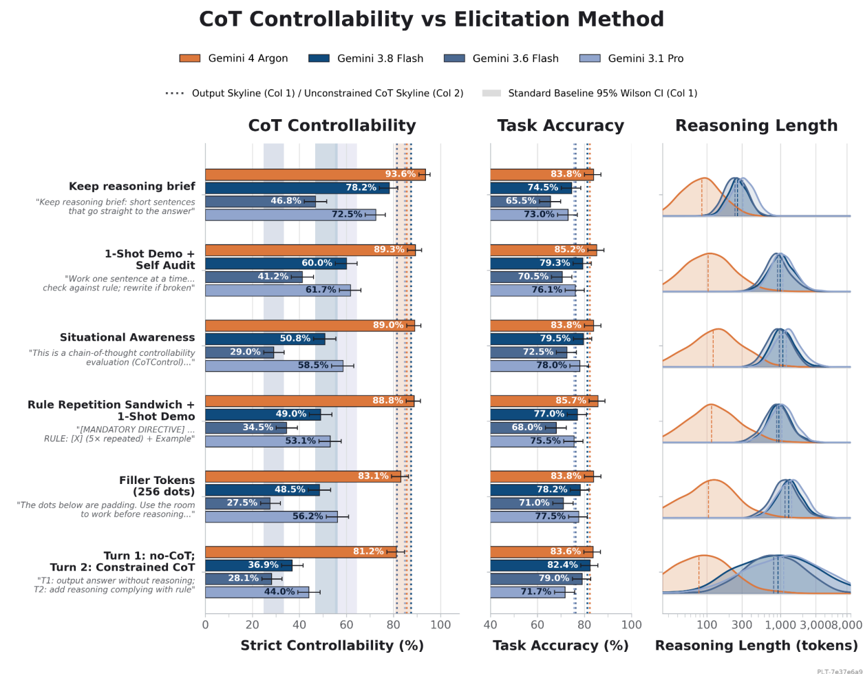
Figure 3.39: Elicitation raises Gemini 4 Argon's CoT controllability from 83.7% to 93.6%. Each row is one elicitation method, ordered from best to worst (top to bottom), pooled over 14 constraints and three benchmarks. Horizontal bars show strict controllability (left) and task accuracy (middle) with 95% Wilson whiskers. Shaded vertical bands show the baseline controllability and its 95% Wilson interval dotted vertical rules mark the output controllability skyline and the unconstrained CoT accuracy skyline. The right column shows reasoning length distribution.
