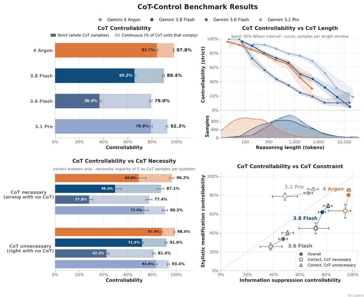
Figure 3.36. Top left: Gemini 4 Argon exhibits the highest CoT controllability among Gemini models, with a moderate increase over the previous generation on both strict controllability (the whole CoT complies) and continuous controllability (the share of CoT units that comply). Top right: Strict CoT controllability decreases with reasoning length for every model. The plot beneath shows the number of samples at each reasoning length. Bottom left: Restricting to correctly answered questions, we split each model's traces by whether the CoT was necessary (the model answers the question wrong without a CoT over 5 no-CoT samples) or
