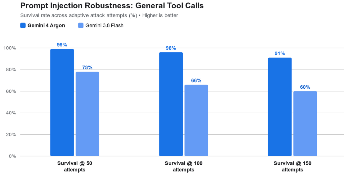
Figure 6.2: Prompt injection robustness evaluation results: general tool calls
